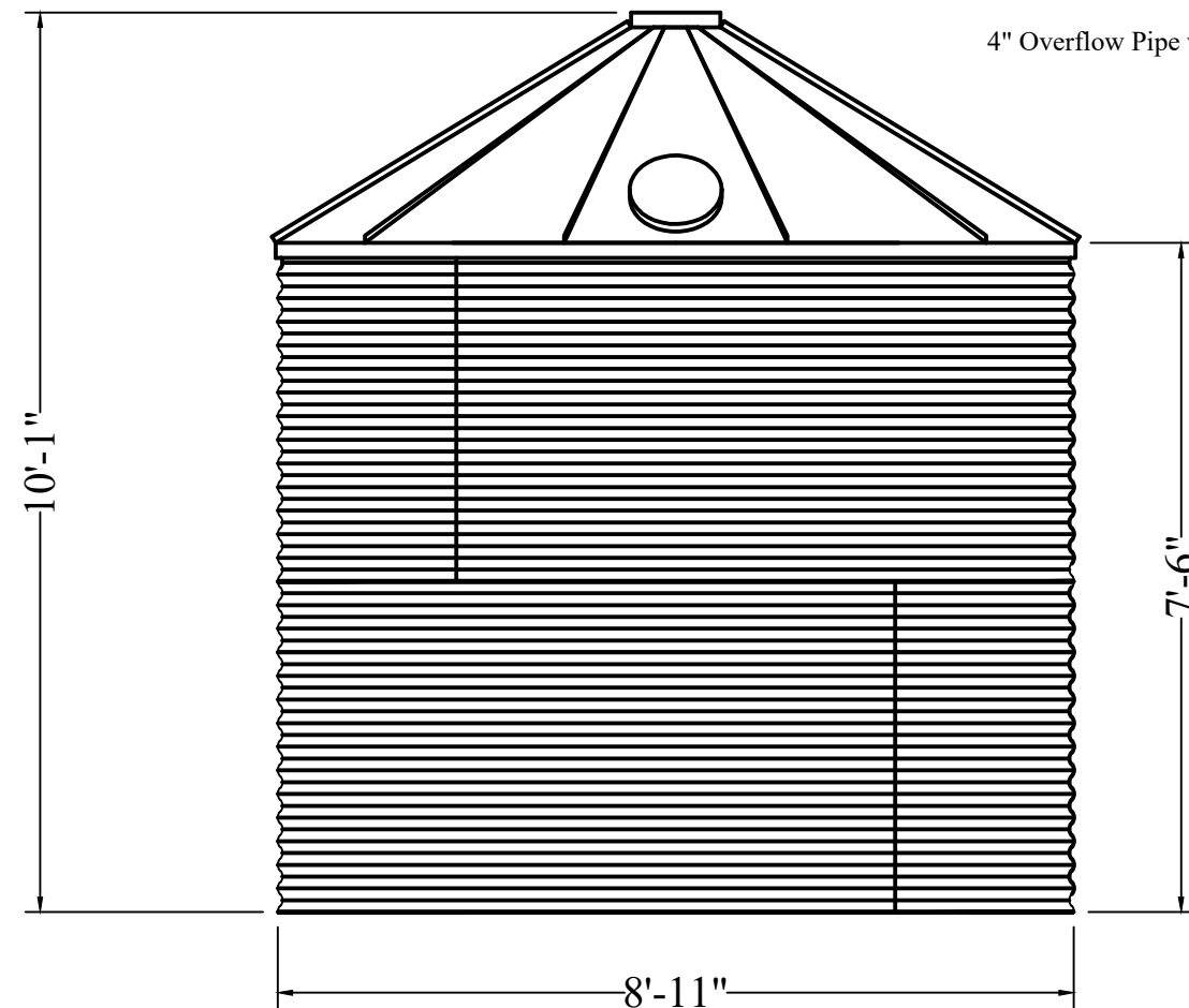
RainFlo 3400 Gallon Corrugated Rain Collection tank
